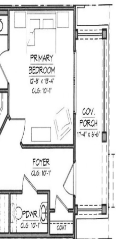
MAIN LEVEL FLOOR PLAN
