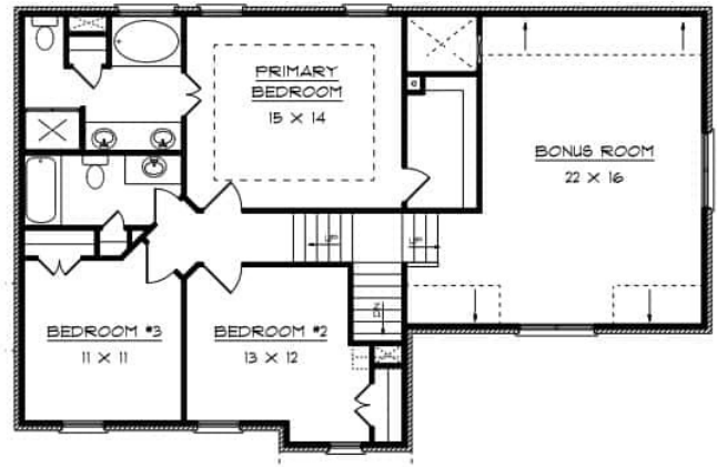
2nd Floor
